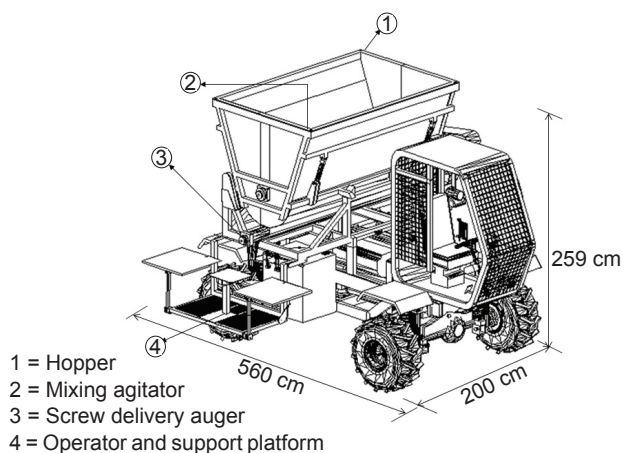
Figure 2. The 3D (three-dimensional) design concept of machine system fully mounted on a 4WD prime mover.
