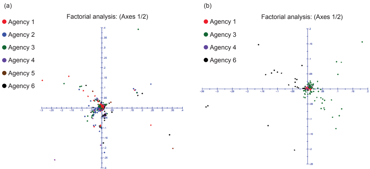
Figure 4. Principal Component Analysis showing coordinates of (a) DxD and (b) TxT individual palms. Dots are coloured corresponding to the six oil palm agencies. Most palms are located close to the centre of PCA. No clear groupings are observed.
