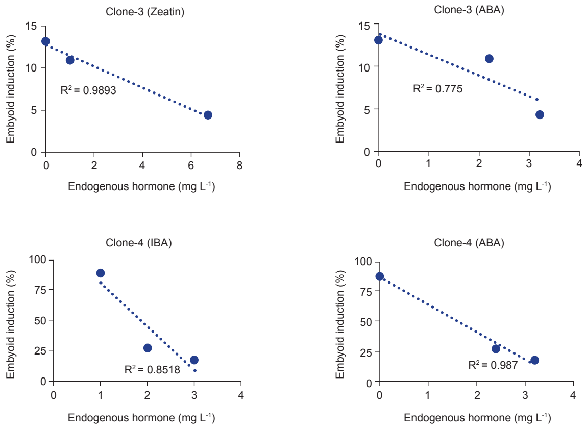
Figure 10. Correlation of endogenous hormones with the percentage of embryoid formation in clone-3, and clone-4.
