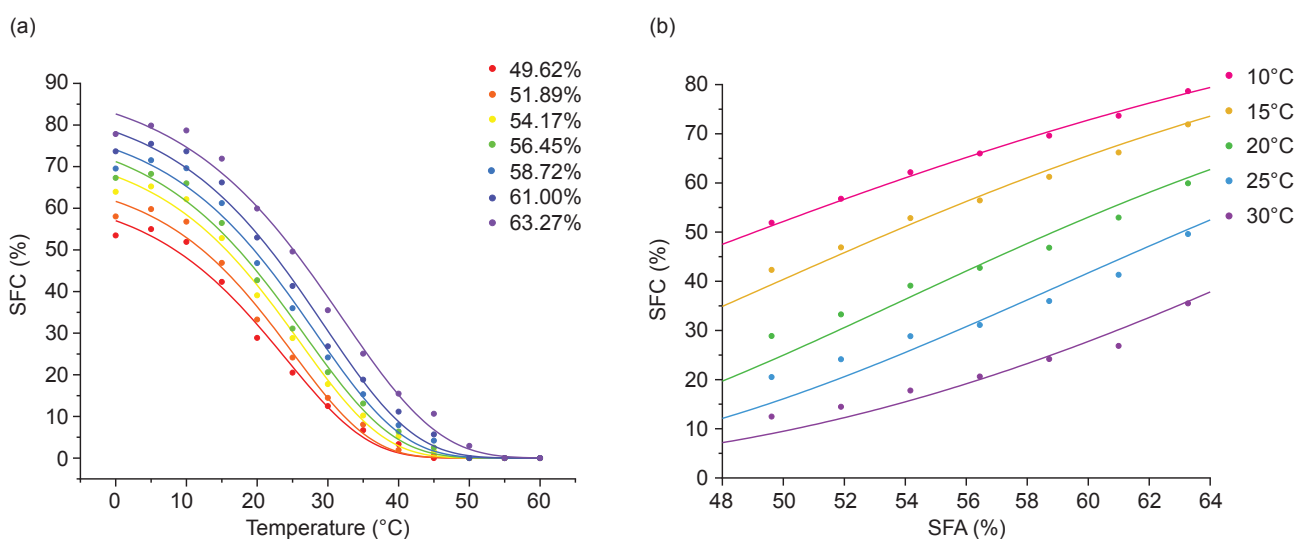
Figure 1. Gompertz fitting curves for the solid fat content (SFC) curves of interesterified binary blends as (a) a function of temperature ( SFC_{f(T)} ) and (b) saturated fatty acids (SFA) ( SFC_{f(SFA)} ). The dashed dots reflect the experimental results, and the lines show the corresponding fitting results.
