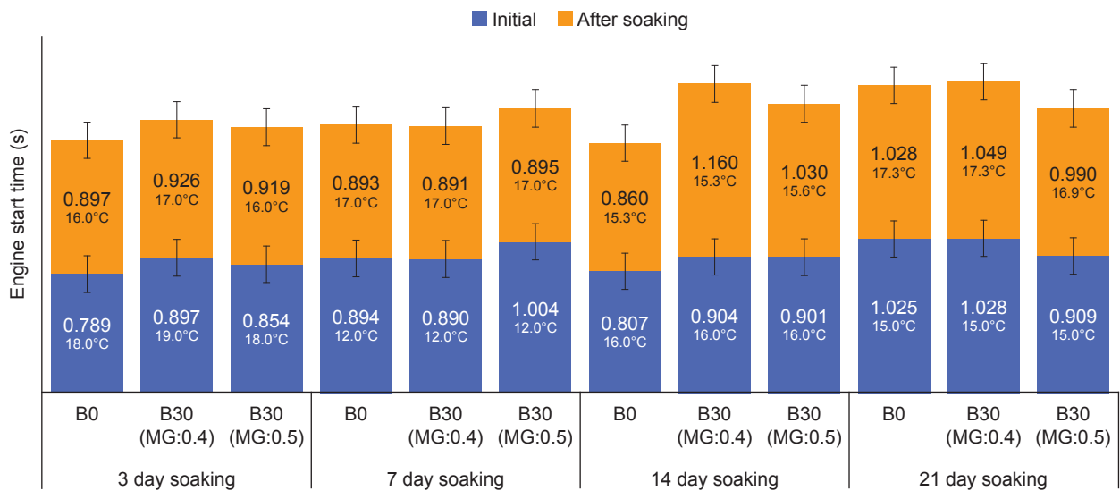
Figure 8. Cold start ability at various soaking period at low ambient temperature.
