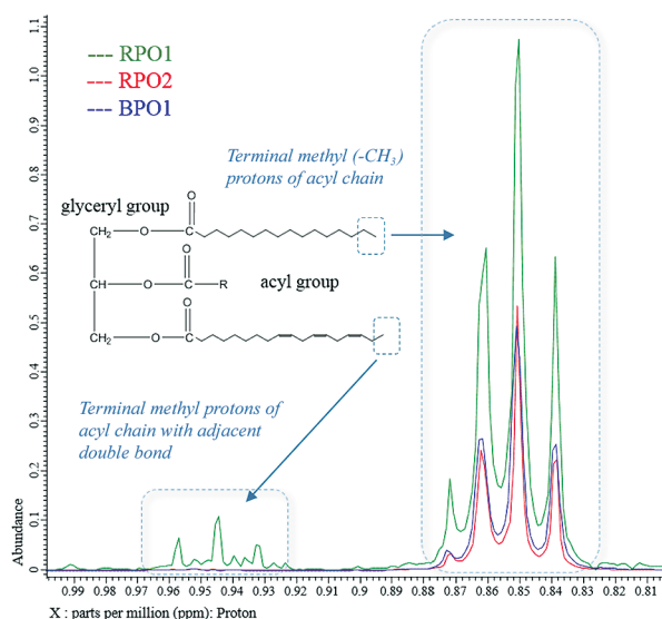
Figure 2. Traces of proton signals at shift 0.93-0.96 ppm in RPO1 proton spectra compared to RPO2 and BPO1 denoting the terminal methyl ( -\text{CH}_3 ) group of linolenic acid.
