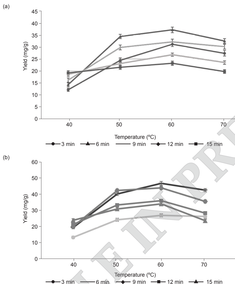
Figure 4. Yield of ferulic acid extracted from sterilised fruitlets using (a) ChCl-CA and (b) ChCl-AA containing 30 wt.% water at different heating duration and temperatures.
