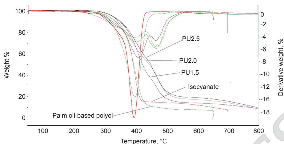
Figure 2. TGA and DTG thermograms of isocyanate, palm-based polyol and palm oil-based PU binders (PU1.5, PU2.0 and PU2.5).
