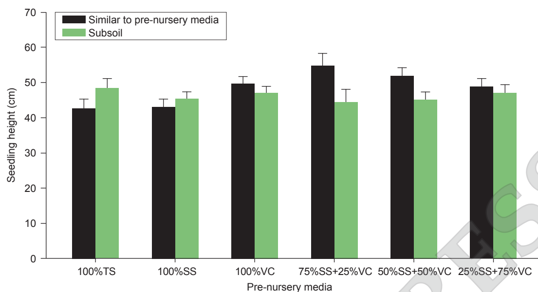
Figure 2. Effect of planting media in the pre-nursery and main-nursery on the height growth of 24-week-old oil palm seedlings in the main-nursery.
