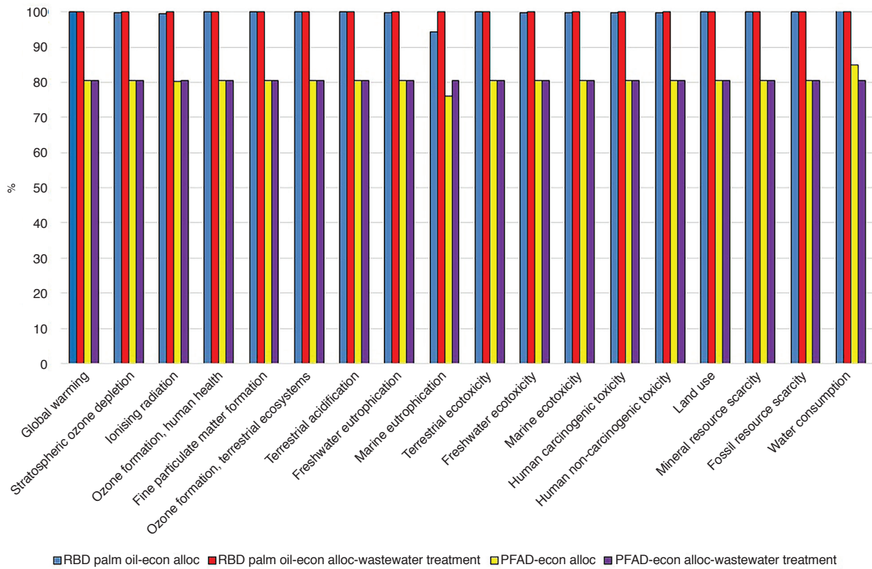
Figure 10. The effects of wastewater treatment to the characterised life cycle impact assessment (LCIA) for the crude palm oil refining.
