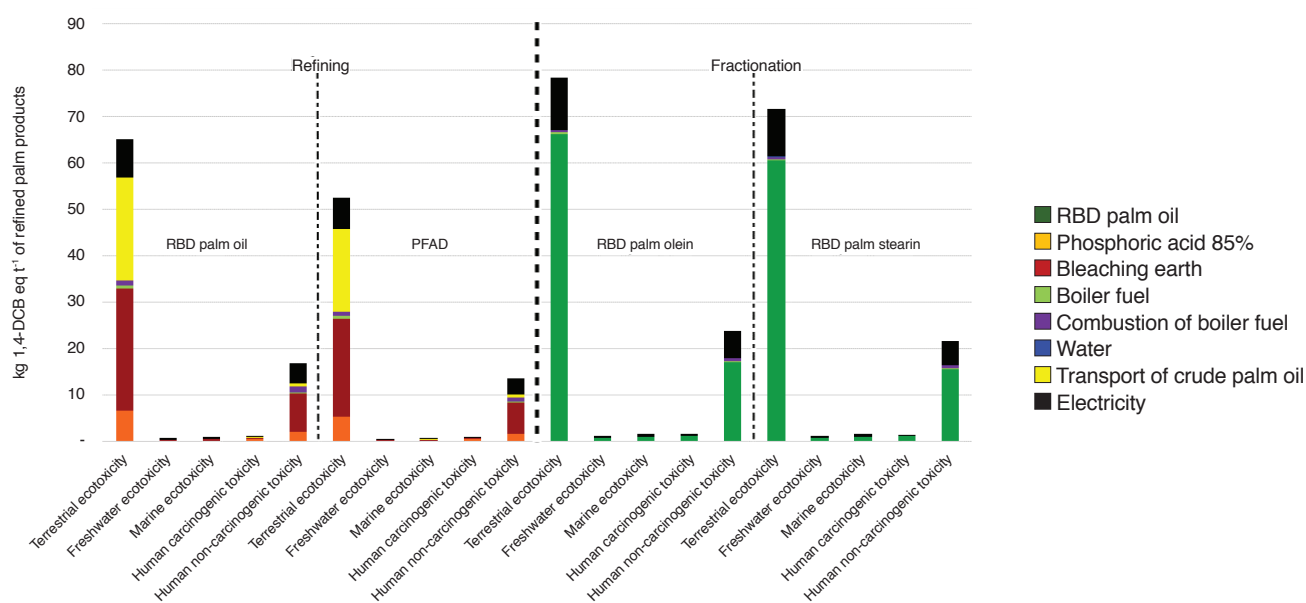
Figure 7. Terrestrial acidification potential for the production of 1 t of refined palm products.
