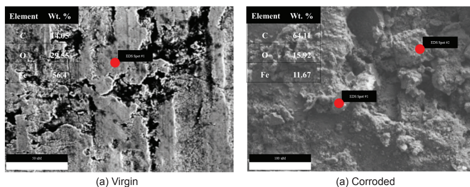
Figure 4. The SEM images of (a) virgin and (b) corroded samples after exposure to B100 biodiesel for 15 years.
